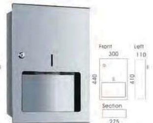
Product Item No. 16K11204 Stainless steel Paper dispenser Size: L300xW110xH440mm
